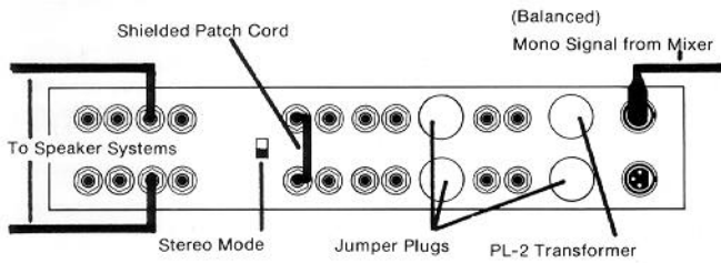
CS-1200 PATCH DIAGRAM 3 Monaural Operation Balanced Low Z Inputs (Jumped Inputs)
